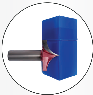
Three Dimensional V-Bit Letter Cutting Bit 32MM 6*32*150° - 6*32*120°
